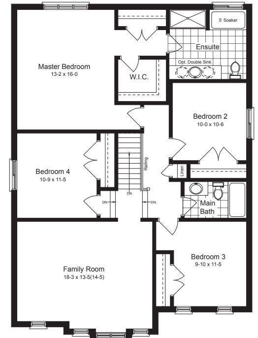
SECOND FLOOR 4 Bedroom Plan
