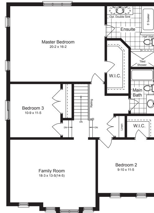
SECOND FLOOR 3 Bedroom Plan
