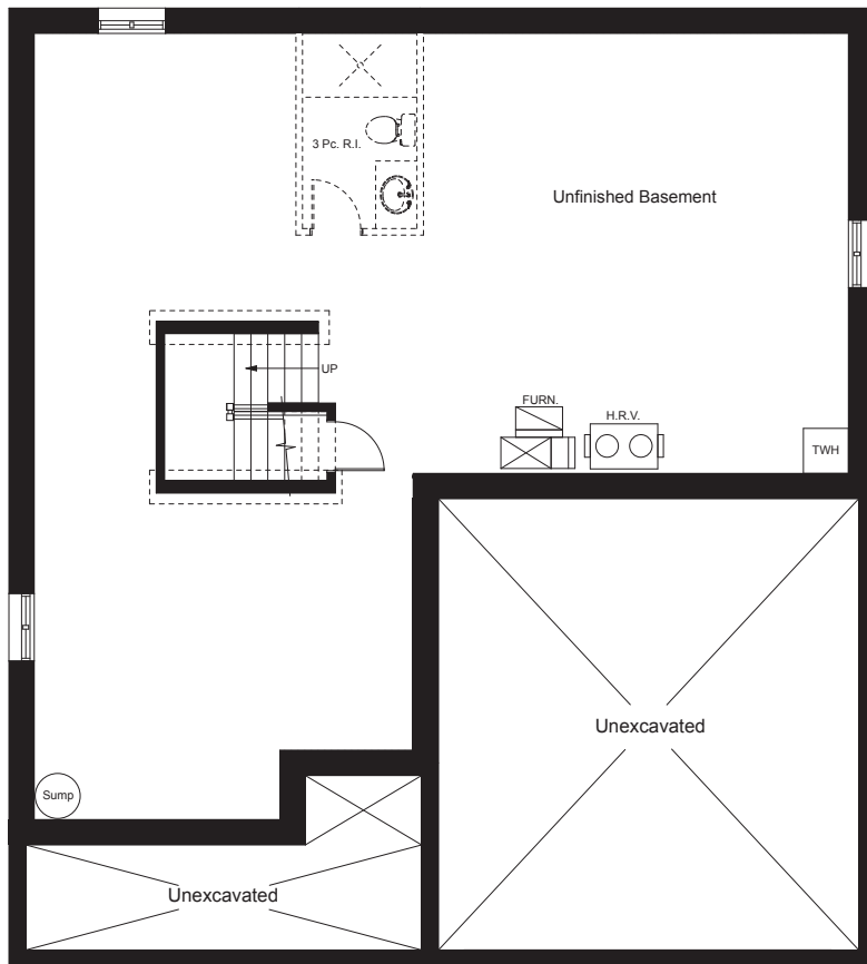
BASEMENT
