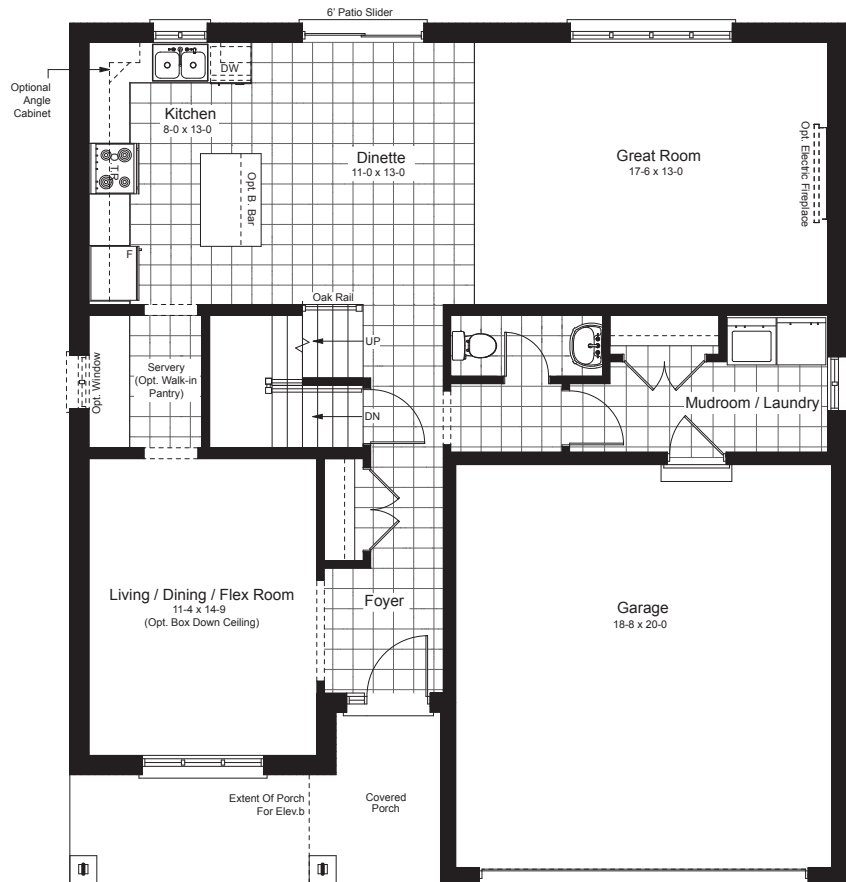
MAIN FLOOR
