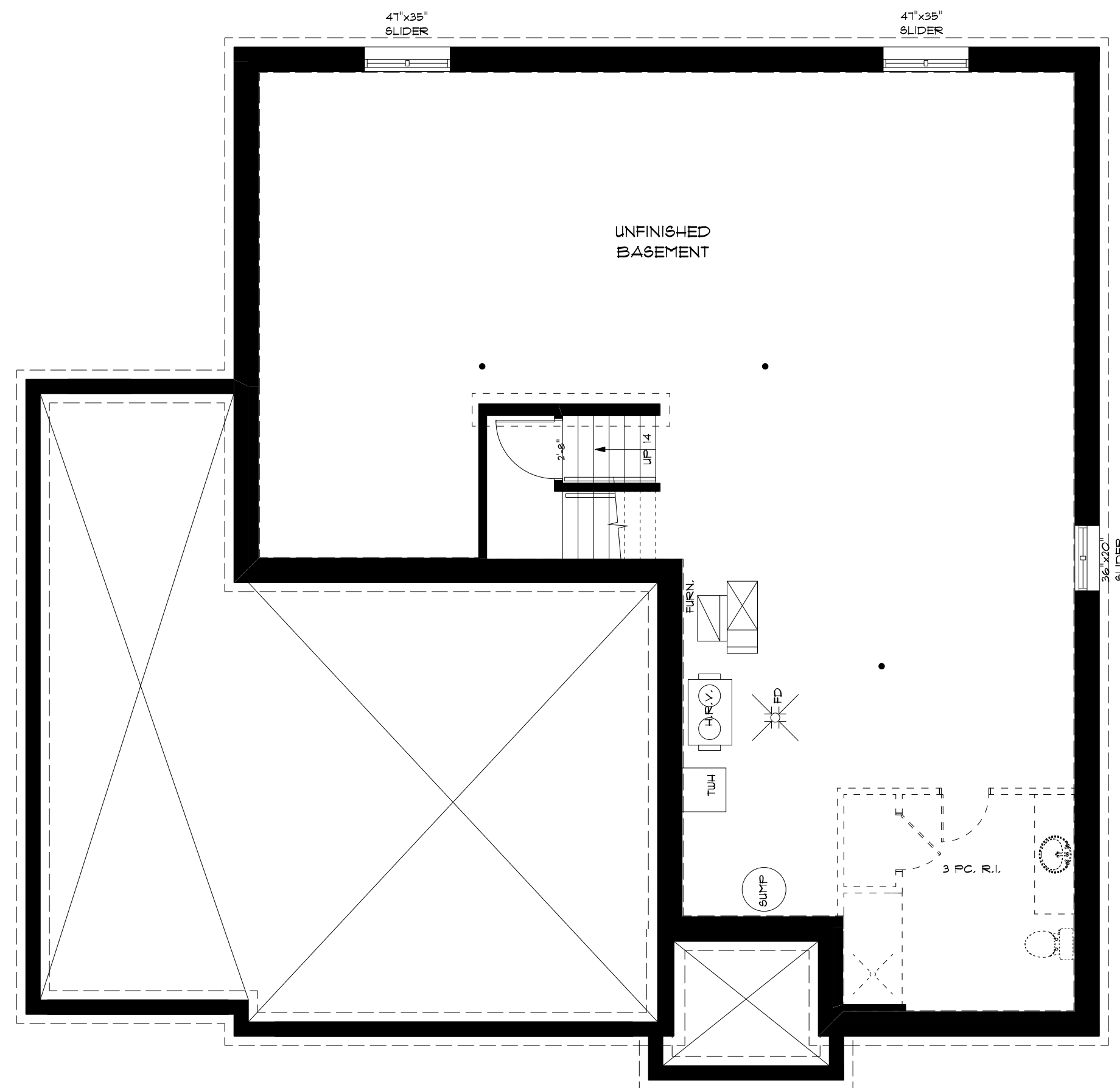
FOUNDATION PLAN
