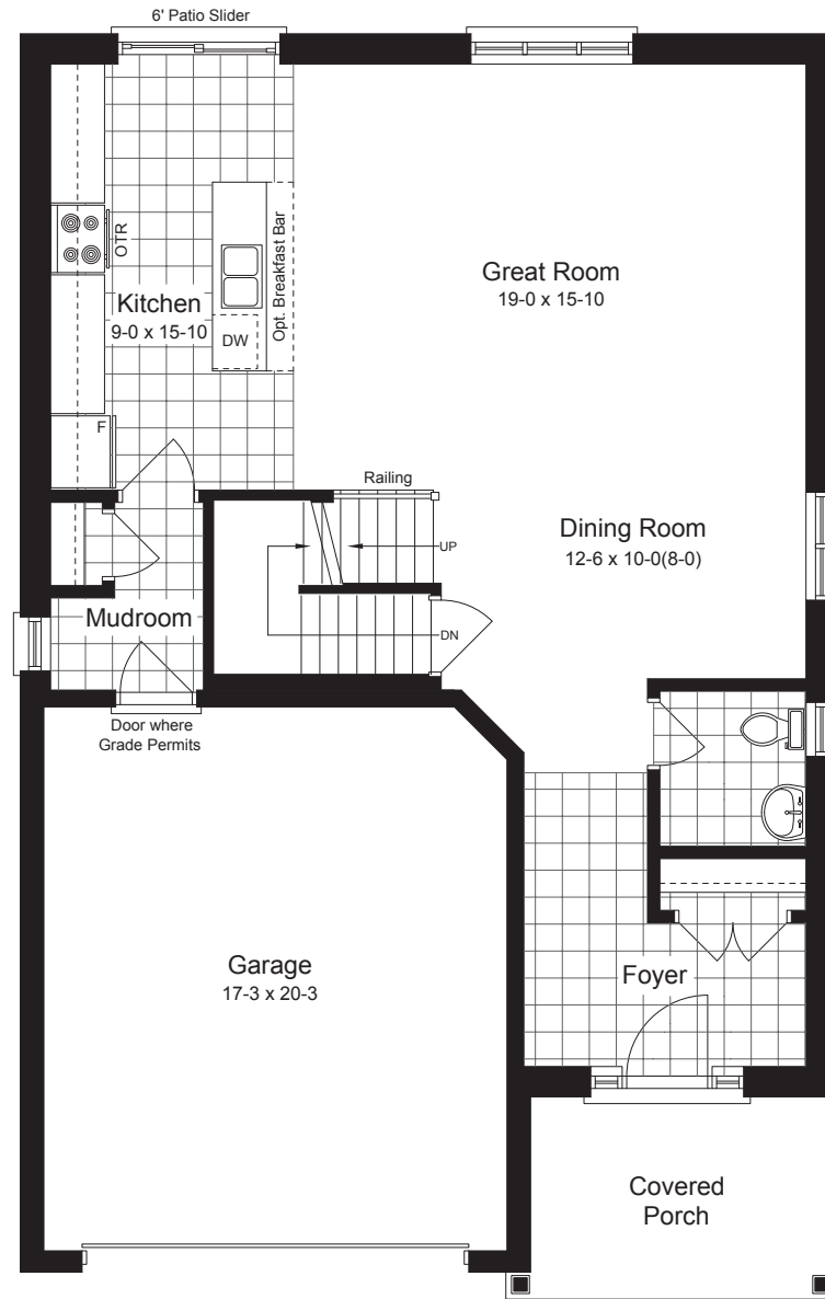
MAIN FLOOR
