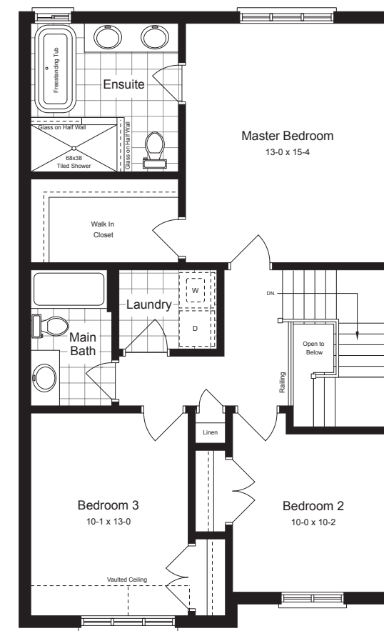
SECOND FLOOR Optional Luxury Ensuite Layout
